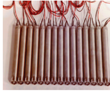
Piezoelectric Diesel injector Actuator
